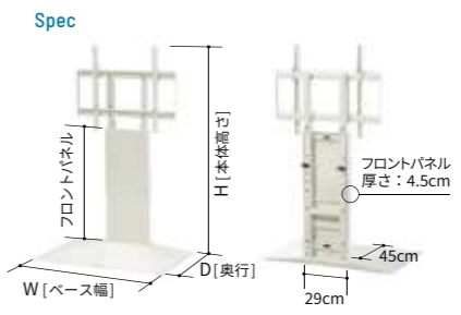
PRODUCT INFO. V4 FLOOR TYPE / COLOR: WALNUT / TV size: 90inch / OPTION: LED LIGHT & SOUNDBAR SHELF LL size
